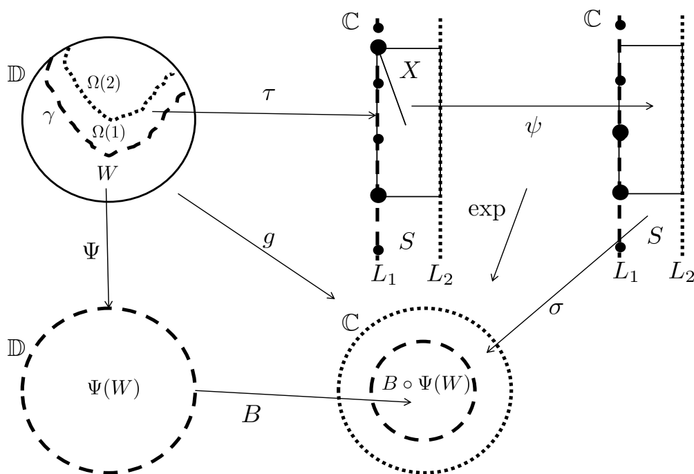
Figure 2. The full interpolation between B \circ \Psi and F . On L_1 , elements of \mathcal{J} are shown as small dots, and two elements of \mathcal{L} are shown as large dots. After the function \psi these elements of \mathcal{L} are coincident with elements of \mathcal{J} .
