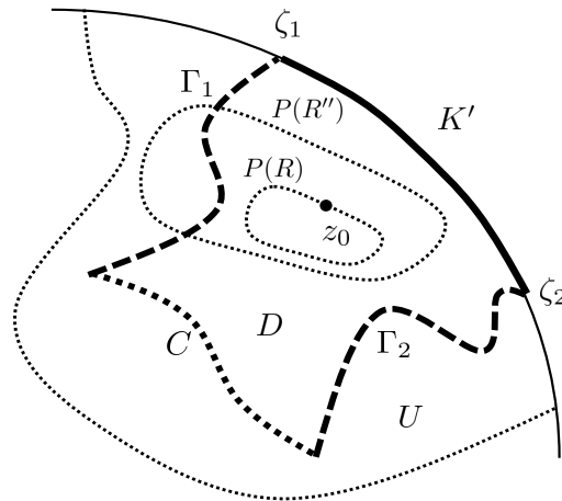
Figure 1. An illustration of the sets in the proof of Theorem 6.
