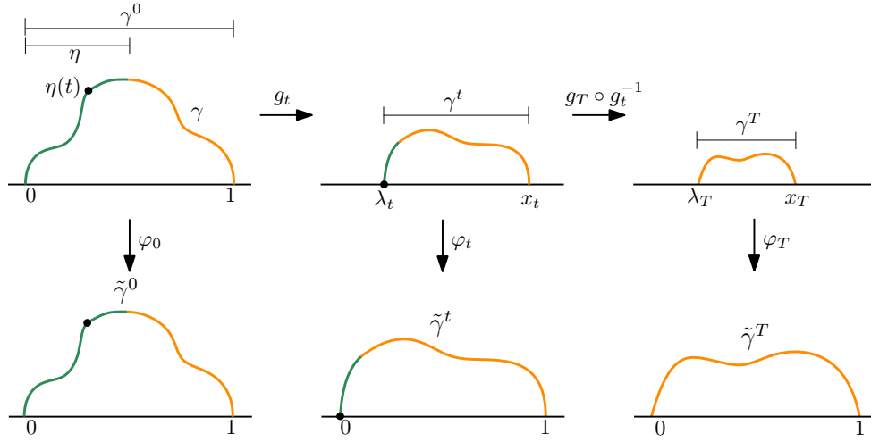
Figure 1. A pictorial description of the proof of Lemma 3.1. Let (g_t)_{t \in [0, T]} be the Loewner chain mapping out \eta , and denote by \gamma^t the chord remaining after mapping out \gamma \cup \eta by g_t . Let \tilde{\gamma}^t be the image of \gamma^t under an affine transformation that maps the endpoints of the chord to 0 and 1. The hulls enclosed by \gamma^t converges in the Carathéodory topology to that enclosed by \gamma^T , and the chords \tilde{\gamma}^t converge along a subsequence to some \tilde{\gamma}^* \in \mathcal{X}(\mathbb{H}; 1, 0) in Hausdorff distance. We have \tilde{\gamma}^* = \varphi_T(\gamma^T) from Lemma 2.6.
