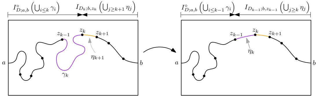
Figure 2. An orientation reversal step in the proof of Proposition 3.4. Left: The curves \gamma_{k+1}, \dots, \gamma_{n+1} to the right of z_k have been replaced with \eta_{k+1}, \dots, \eta_{n+1} in the previous steps. The orange curve \eta_{k+1} is a hyperbolic geodesic in the complement of black and purple parts of the chord. Right: We replace the purple curve \gamma_k with a hyperbolic geodesic \eta_k in the complement of black and orange parts of the chord. The total energy of the curves in the right figure is no more than that in the left figure. Moreover, if \gamma_k \neq \eta_k , then the inequality is strict.
